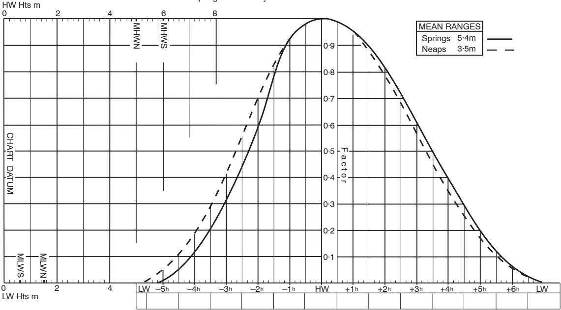
DUNKERQUE MEAN SPRING AND NEAP CURVES Springs occur 2 days after New and Full Moon.
