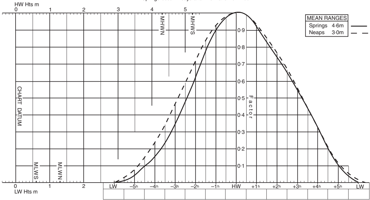
OOSTENDE MEAN SPRING AND NEAP CURVES Springs occur 2 days after New and Full Moon
